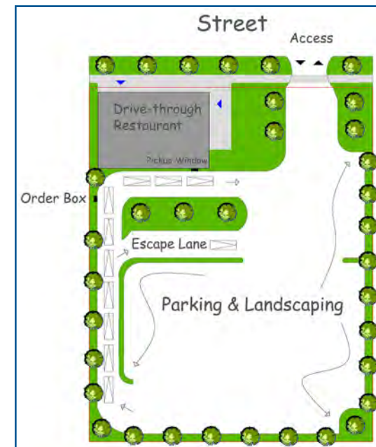
Figure 4.6a: Sketch showing an uninterrupted linear stacking lane and an escape lane that allows vehicles to exit without having to drive by the pickup window.
